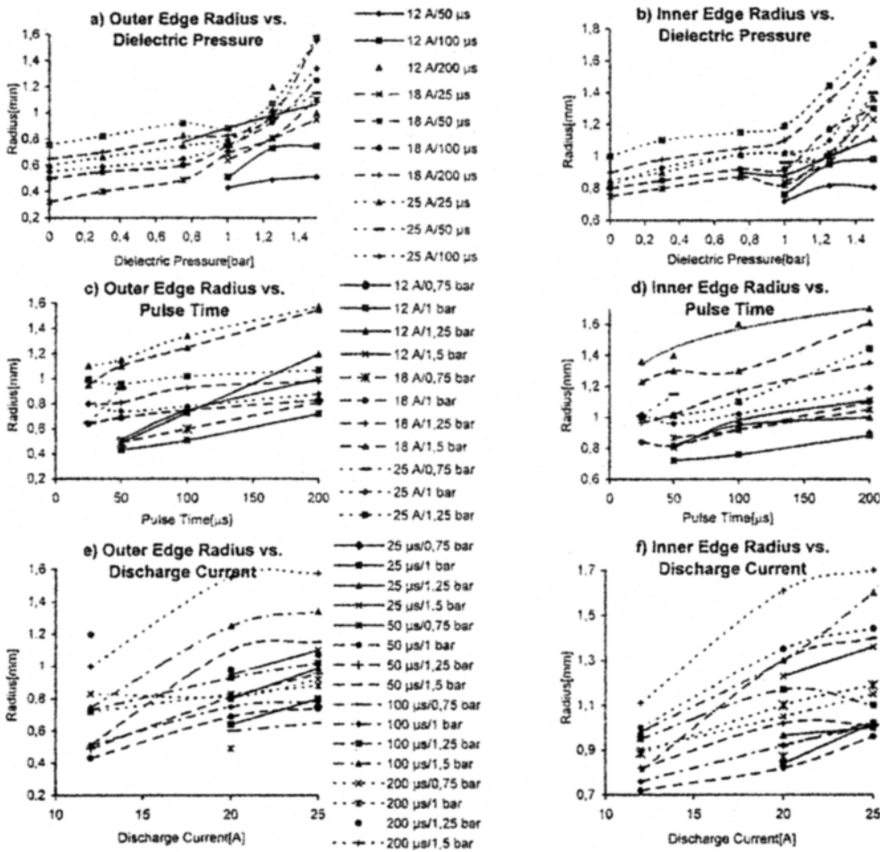
Fig. 5 Variation of edge radius with machining parameters
