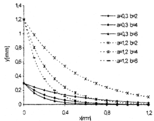
Fig. 6 Various shapes of the exponential model
